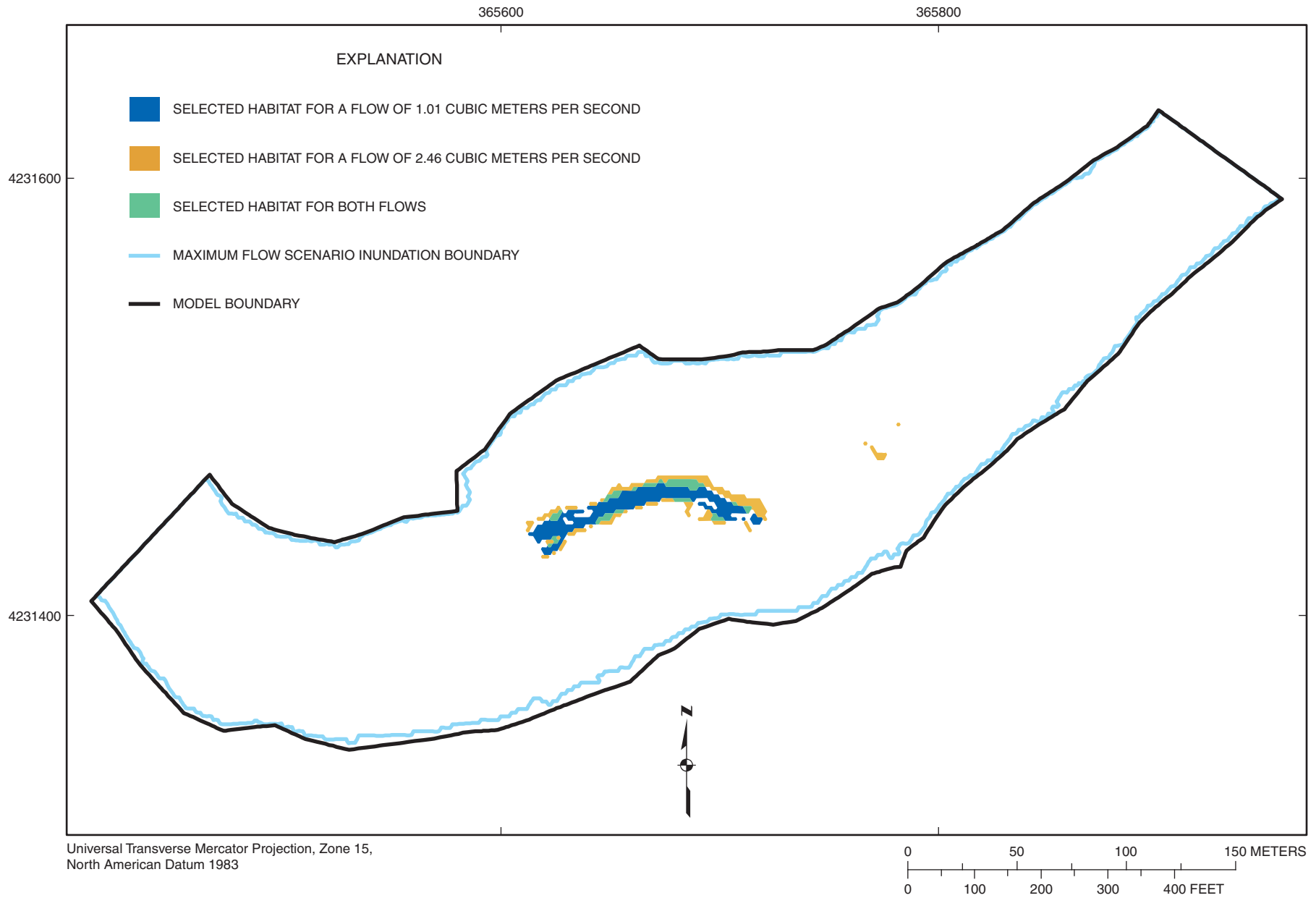
Figure 4-77. Selected habitat area distribution for habitat category 20 (flathead catfish) at flows of 1.01 and 2.46 cubic meters per second at Marais des Cygnes River site MDC2.
